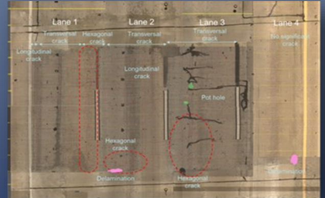
Overall condition of the deck at downtown
